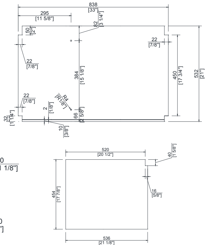
Solid Wood Construction Bathroom Vanity
