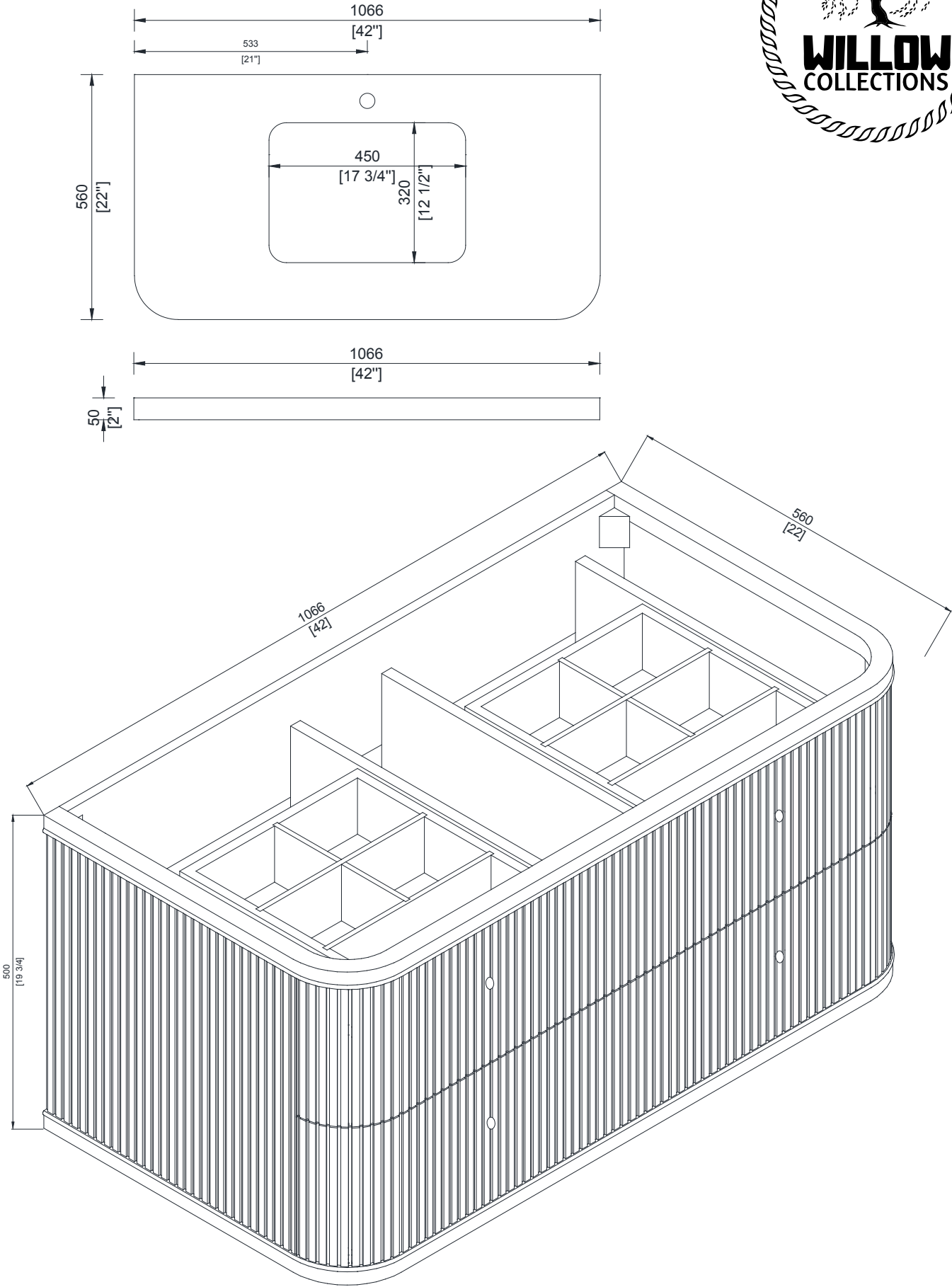
Solid Wood Construction Bathroom Vanity
