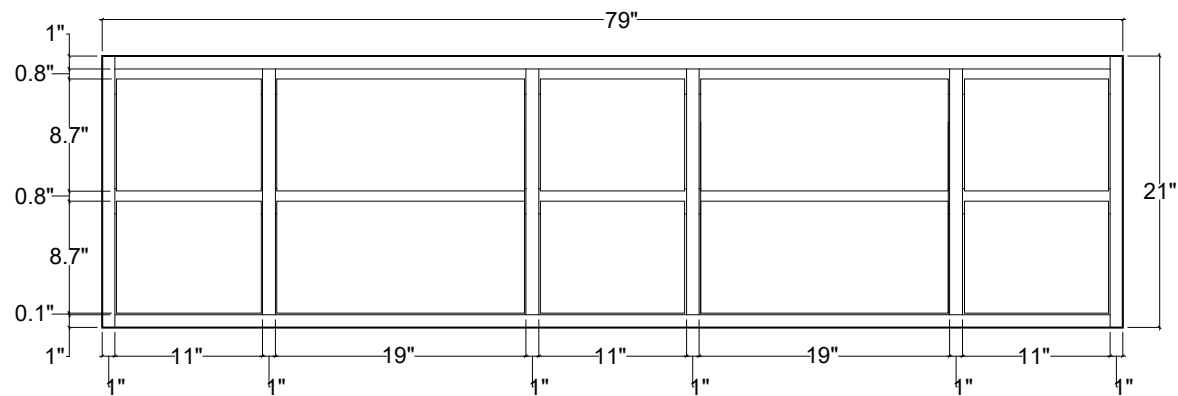
FRONT VIEW
