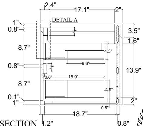
SIDE SECTION
