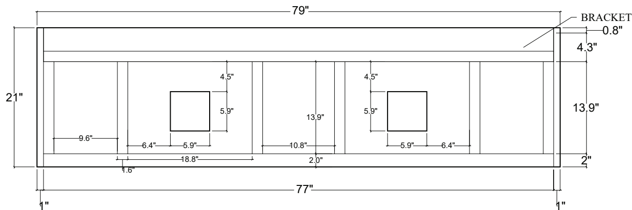
BACK VIEW
