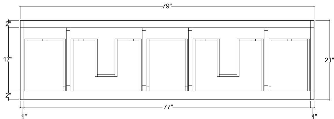
TOP VIEW
