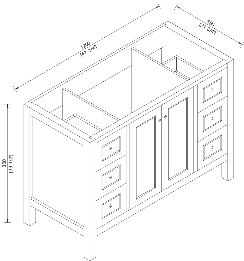
Solid Wood Construction Bathroom Vanity
