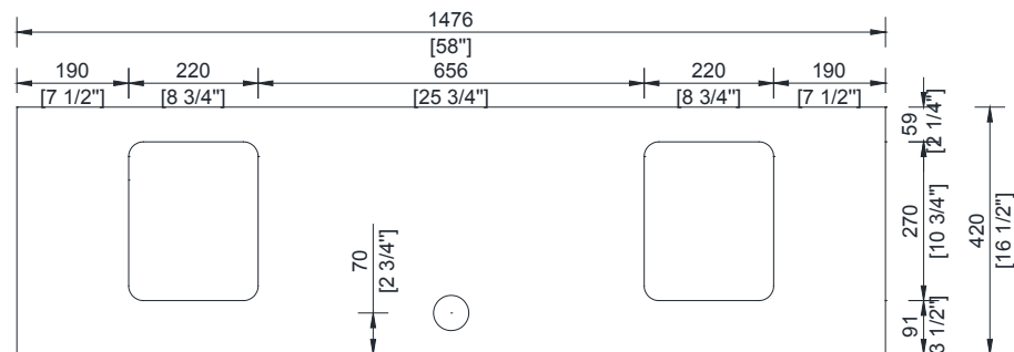
Solid Wood Construction Bathroom Vanity
