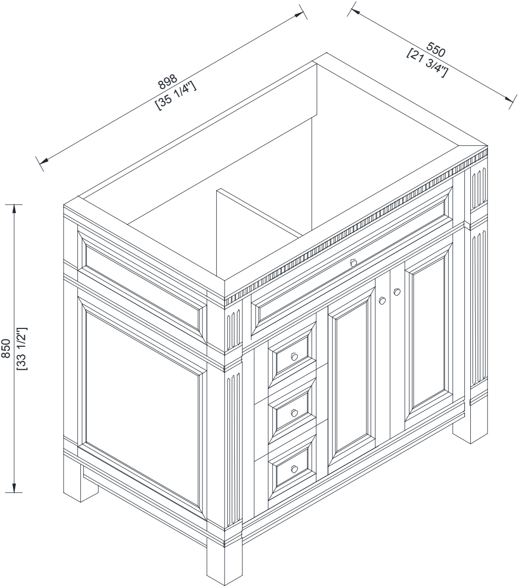
Solid Wood Construction Bathroom Vanity
