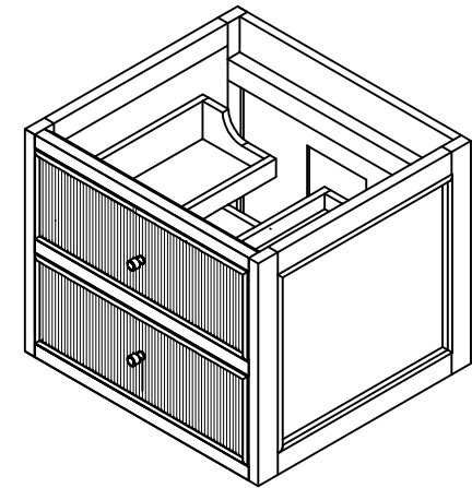
ISOMETRI VIEW
