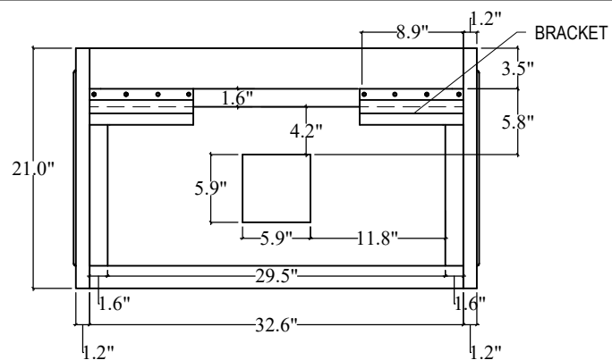
BACK VIEW
