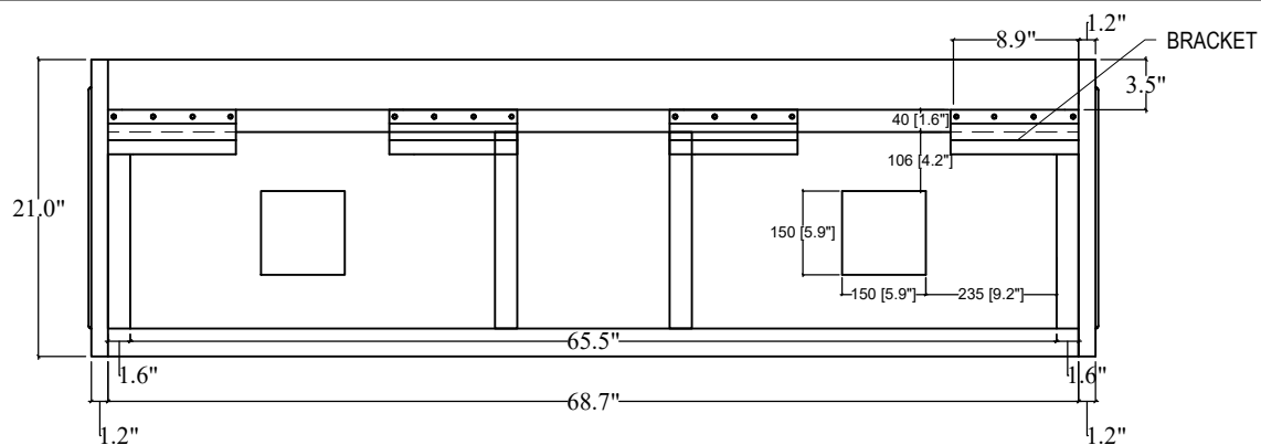
BACK VIEW
