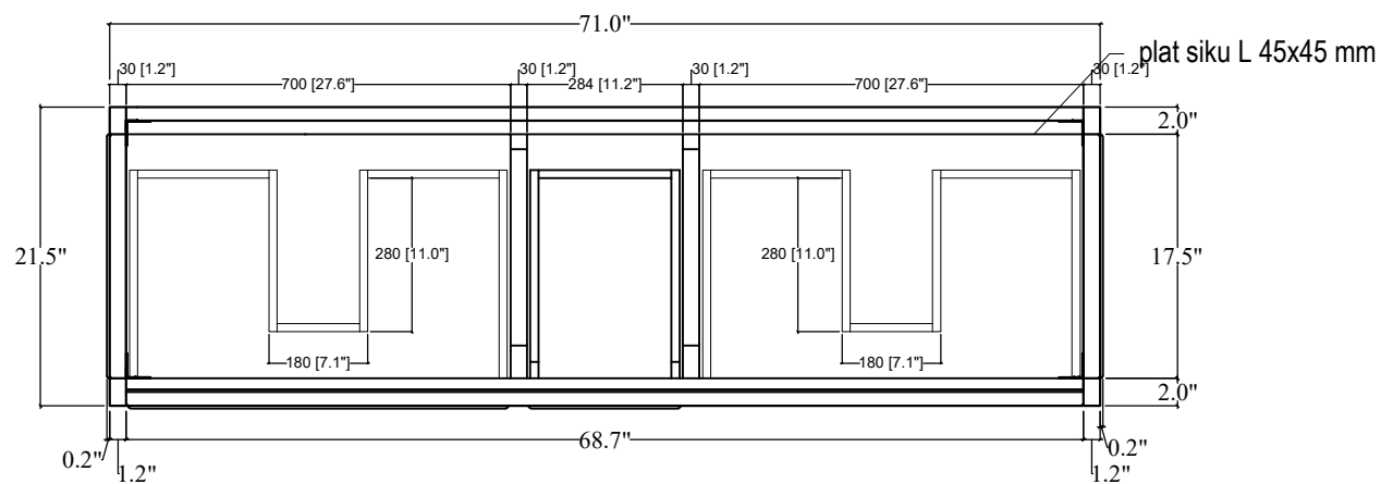
TOP VIEW
