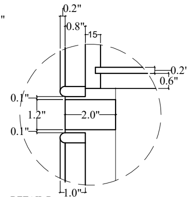
DETAIL B
