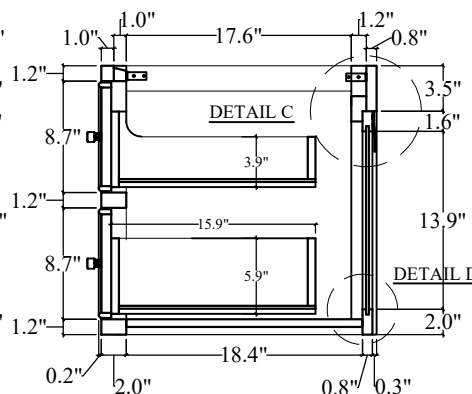
SECTION C-C
