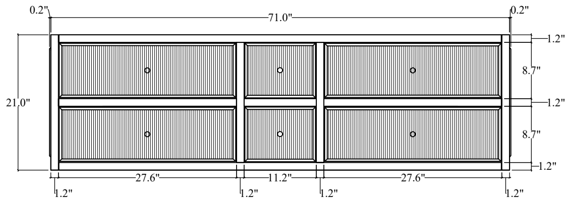
FRONT VIEW
