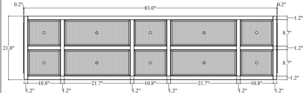
FRONT VIEW
