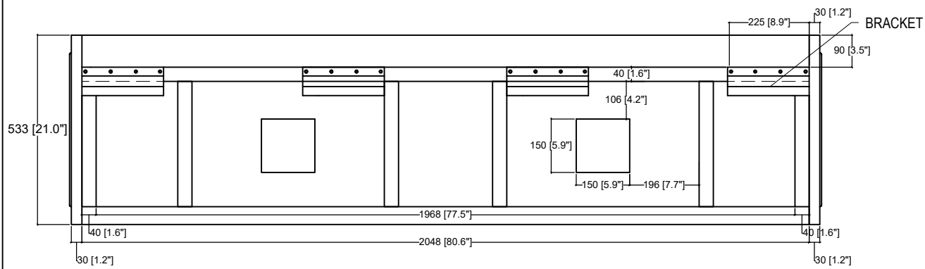
BACK VIEW
