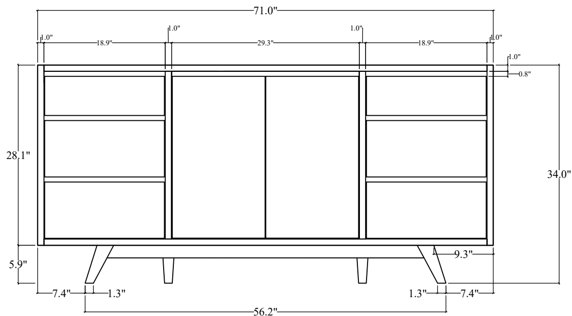
FRONT VIEW
