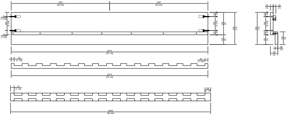
39-66*86寸床:1600*2122*1219 ( H )
